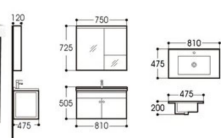
PV3002-80 BATHROOM CABINET Main cabinet Size: 810x475x505mm Mirror cabinet Size: 750x120x725mm Ceramic basin Size: 810x475x200mm Material: PVC
