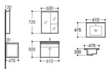
PV3001-60 BATHROOM CABINET Main cabinet Size: 610x475x505mm Mirror cabinet Size: 600x120x725mm Ceramic basin Size: 610x475x200mm Material: PVC
