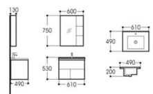
PW1002-60 BATHROOM CABINET Main cabinet Size:610x490x530mm Mirror cabinet Size:600x130x750mm Ceramic basin Size:610x490x200mm Material: plywood
