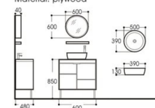
PW1005-60 BATHROOM CABINET Main cabinet Size:600x480x850mm Mirror Size:600x40x600mm Shelf Size:600x130x40mm Ceramic basin Size:500x390x130mm Material: plywood
