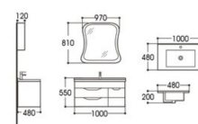
CP968 BATHROOM CABINET Main cabinet Size: 1000x480x550mm Mirror cabinet Size: 970x120x810mm Ceramic basin Size: 1000x480x200mm Material: PVC
