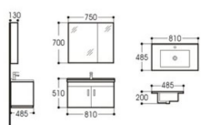
PW1003-80 BATHROOM CABINET Main cabinet Size:810x485x510mm Mirror cabinet Size:750x130x700mm Ceramic basin Size:810x485x200mm Material: plywood
