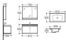
PW1001-80 BATHROOM CABINET Main cabinet Size:810x500x530mm Mirror cabinet Size:750x130x700mm Ceramic basin Size:810x500x200mm Material: plywood
