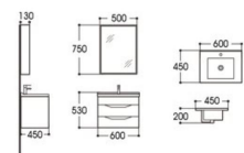
CP966 BATHROOM CABINET Main cabinet Size: 600x450x530mm Mirror Size: 500x130x750mm Ceramic basin Size: 600x450x200mm Material: PVC
