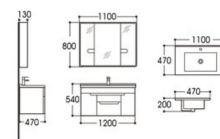
CP969 BATHROOM CABINET Main cabinet Size: 1200x470x540mm Mirror cabinet Size: 1100x130x800mm Ceramic basin Size: 1100x470x200mm Material: PVC
