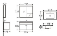
PV3001-80 BATHROOM CABINET Main cabinet Size: 810x475x505mm Mirror cabinet Size: 750x120x725mm Ceramic basin Size: 810x475x200mm Material: PVC
