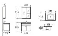
PV3002-60 BATHROOM CABINET Main cabinet Size: 610x475x505mm Mirror cabinet Size: 600x120x725mm Ceramic basin Size: 610x475x200mm Material: PVC
