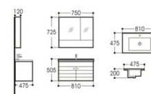
AL2002-80 BATHROOM CABINET Main cabinet Size:810x475x505mm Mirror cabinet Size:750x120x725mm Ceramic basin Size:810x475x200mm Material: aluminum
