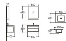
AL2001-60 BATHROOM CABINET Main cabinet Size:600x400x280mm Mirror Size:500x20x690mm Ceramic basin Size:600x400x200mm Material: aluminum
