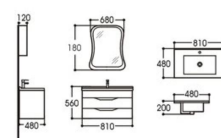
CP967 BATHROOM CABINET Main cabinet Size: 810x480x560mm Mirror cabinet Size: 680x120x180mm Ceramic basin Size: 810x480x200mm Material: PVC
