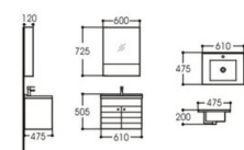
AL2002-60 BATHROOM CABINET Main cabinet Size:610x475x505mm Mirror cabinet Size:600x120x725mm Ceramic basin Size:610x475x200mm Material: aluminum
