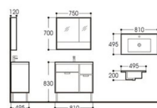
PW1004-80 BATHROOM CABINET Main cabinet Size:810x495x830mm Mirror cabinet Size:750x120x700mm Ceramic basin Size:810x495x200mm Material: plywood
